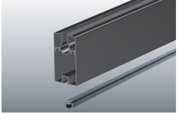
Strong and firm bottom rail with anti-collision rubber strip installed.
